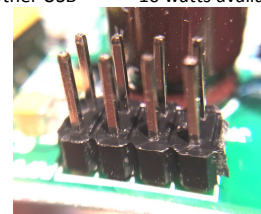
These 4 jumpers enable mode B operation
